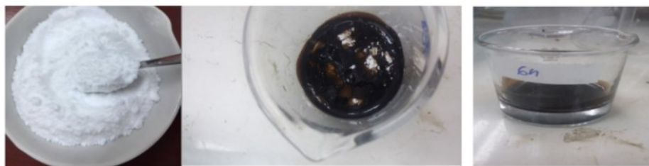
Figure 9. Experimental observation of crude oil adsorption by nanosilica LGP (sample M 2 )
