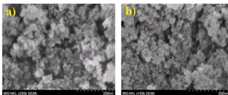
Figure 2. FESEM image of nanosilica LGP sample (sample M_2 )
