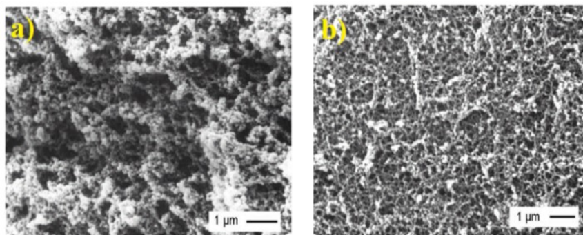
Figure 4. FESEM image of nanosilica LGP sample (Sample M_4 )
