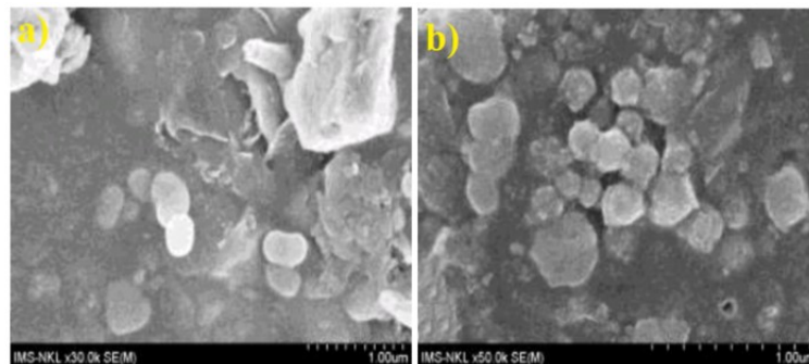
Figure 1. FESEM image of nanosilica LGP sample (sample M_1 )
