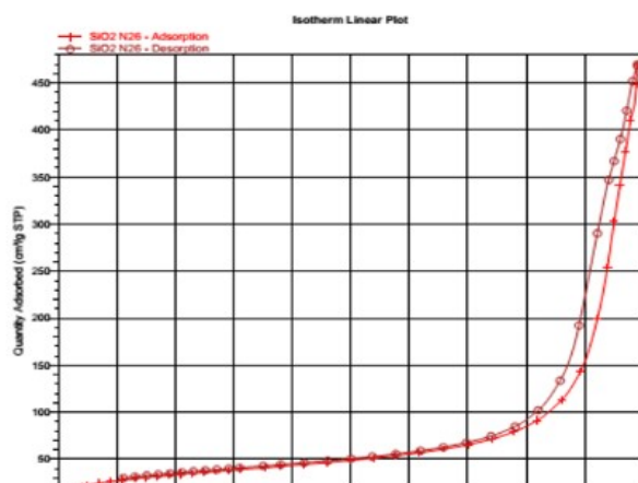
Figure 8. N_2 adsorption–desorption isotherm of nanosilica synthesized from LGP
