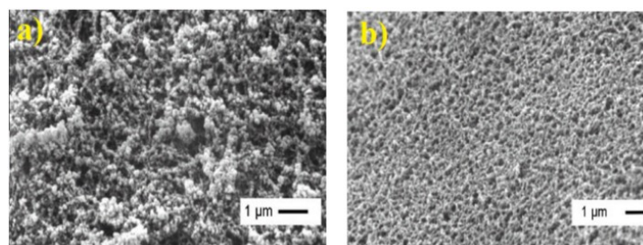
Figure 3. FESEM image of nanosilica LGP sample (sample M_3 )
